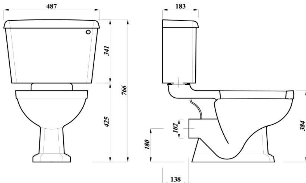
Shown :Close Coupled WC Suite, available with (P) trap, with and without douche.
