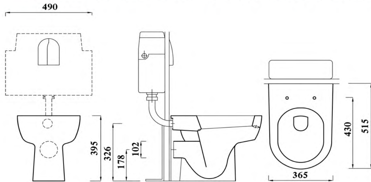
Shown : WC back to wall, available in ( S ) trap. Available without douche.
