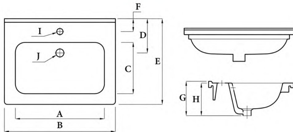
Shown : 60 cm Basin Available with 1 tap hole only with Milano mixer
