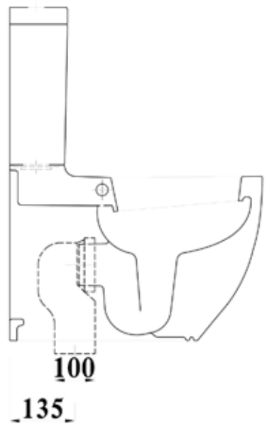
Quartz WC With Tank
