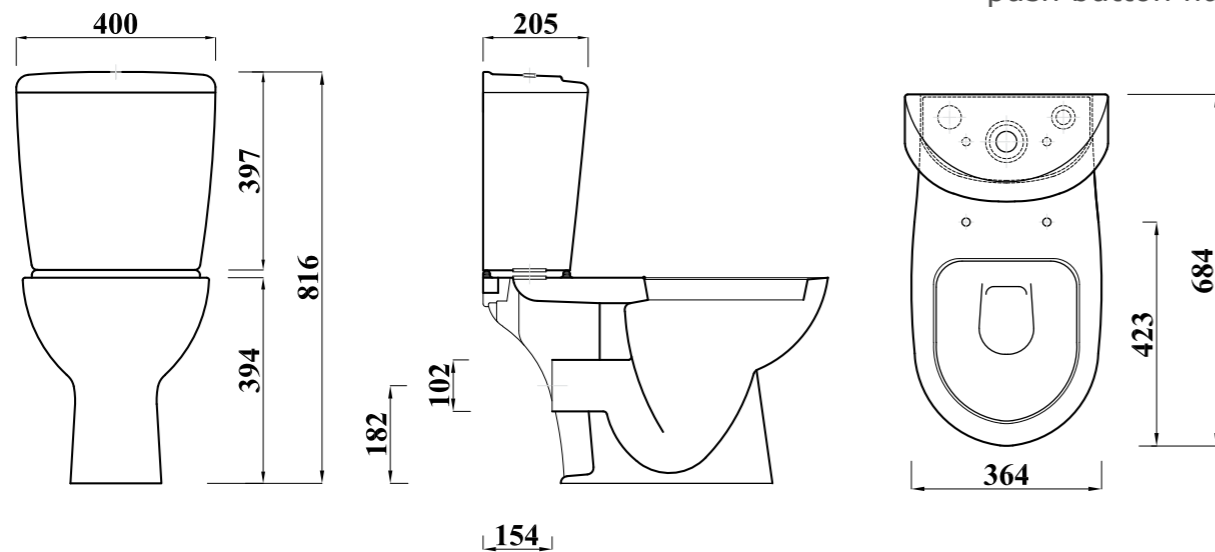
Shown : Close Coupled WC Suite, available in (P & S) trap. With doche, push button flush.
